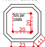
PIANTA art. 819/C
