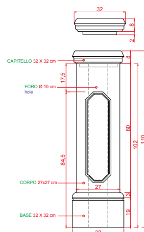
ART. 1271 PILASTRINO GRANDE h cm 110 - base cm 32X32 peso kg 148 43.30' ' tall - 12.59' ' L - 12.59' ' W 326.28 lbs
