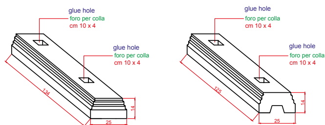
ART. 1214 BASE GRANDE h cm 14x25 - lungh. cm 125 (A) - cm 134 (B) - peso kg 76 5.51"x9.24" tall - 49.21" (A) - 52.75" (B) length - 167.55 lbs
