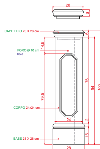
ART. 1271 PILASTRINO GRANDE h cm 110 - base cm 32X32 peso kg 148 43.30" tall - 12.59" L - 12.59" W 326.28 lbs
