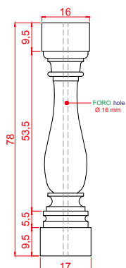
ART. 1238 COLONNETTA SAVOIA h cm 78 - peso kg 29 30.70" tall - 63.93 lbs
